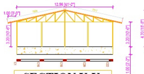
SECTION Y-Y MACHINERY UNIT SHED
