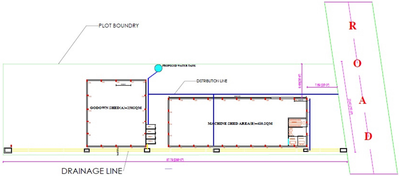
LAYOUT PLAN
